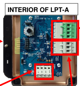
RELAY CONNECTION 2-AMP @30V RELAY OPERATES IN "FAIL SAFE" CONFIGURATION
