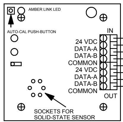
DST SERIES DIGITAL TRANSMITTER WITH SOLID-STATE SENSOR SHOWN
